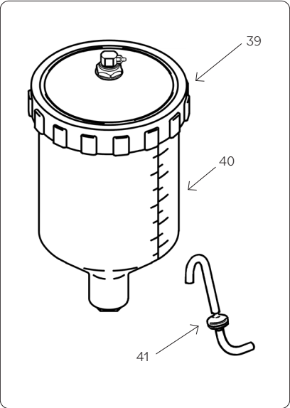
Gravity Cup Assembly (#9860)
