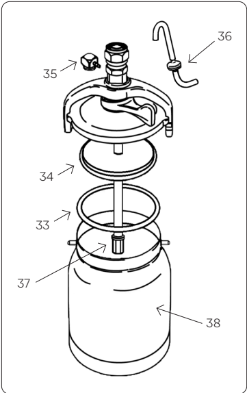
Bottom Feed Cup Assembly (#2095)
