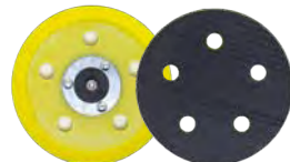
105GV 5" Backup Pad Medium, 5-Hole Grip, 5/16 - 24 thread
