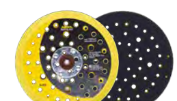
916SGV 6" Backup Pad Soft, Multi-Hole, Grip 5/16" - 24 thread
